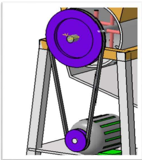
Fig 3.3 Belt and Pulley Drive
