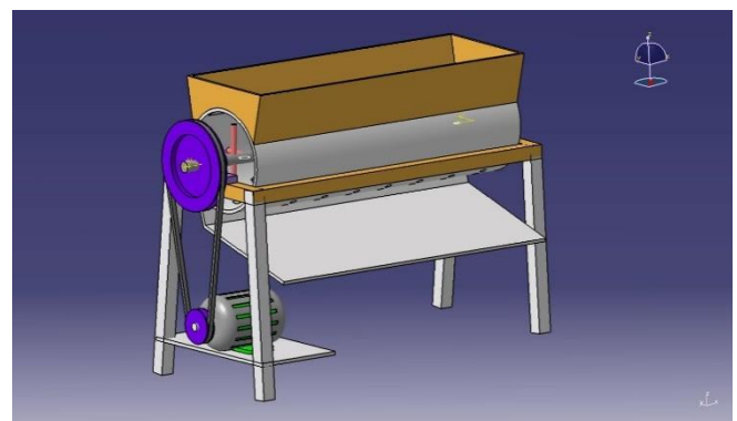
FIG 4.1 ASSEMBLY OF CORN SHELLING MACHINE
