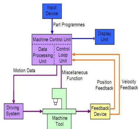
Fig.1. Close loop system
