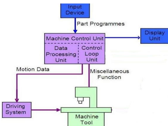
Fig.2. Open loop system
