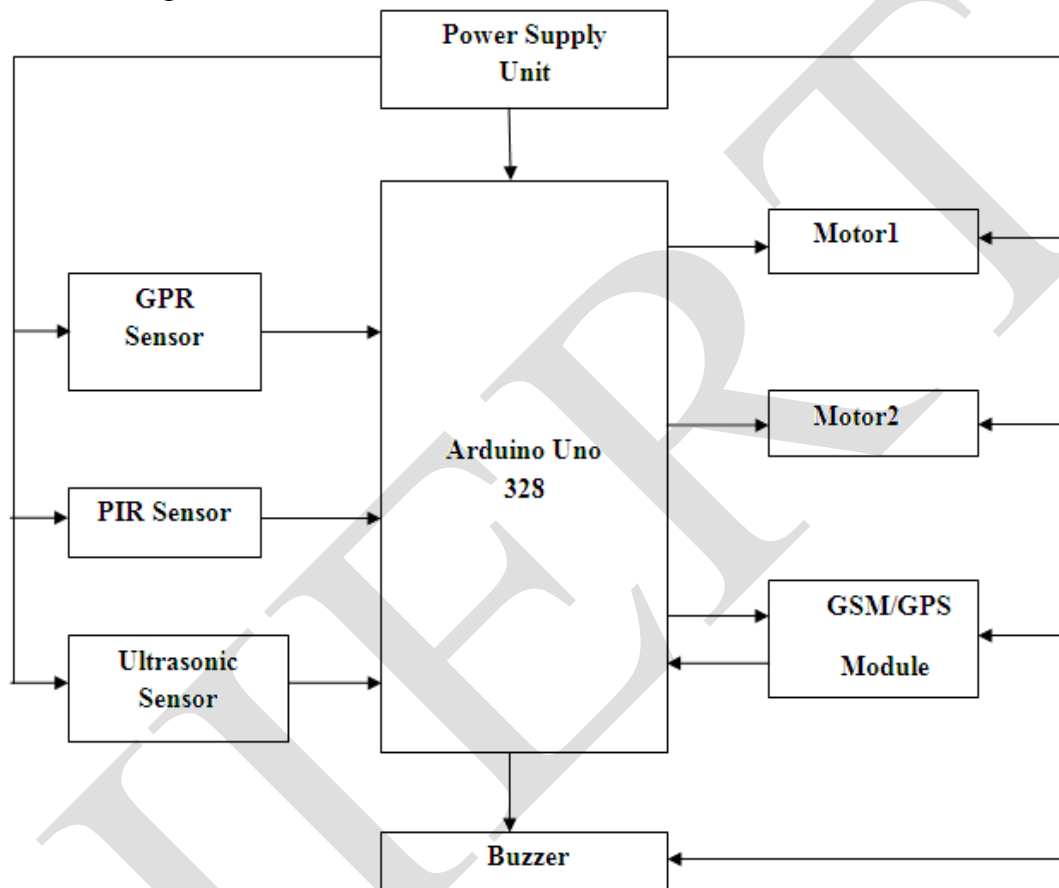
Fig.1. Block Diagram
