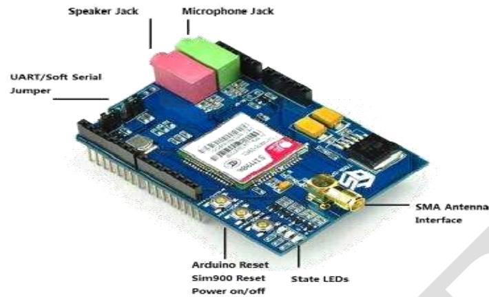
Fig .6 GSM Board
