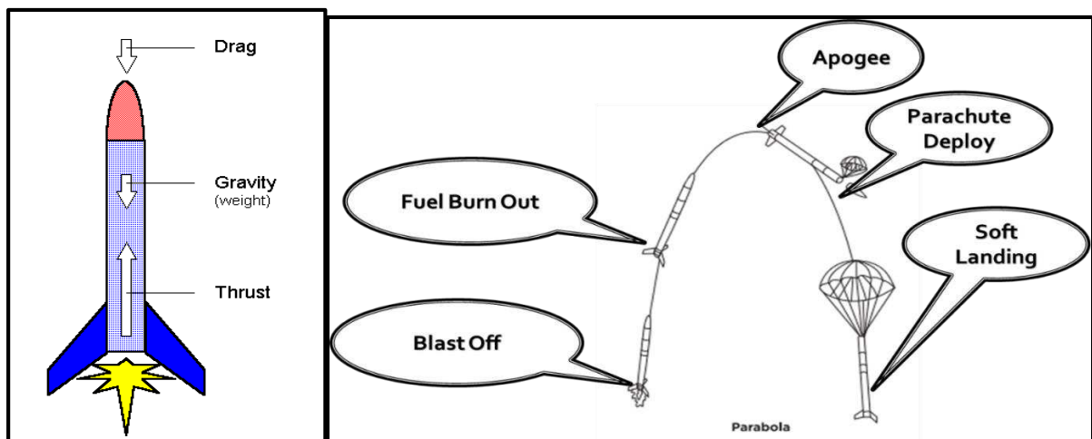
Fig. 4(a) Forces on Rocket
