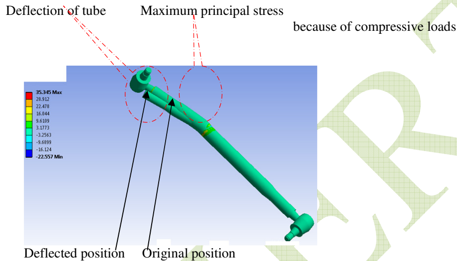
Fig.9 Maximum principal stress
