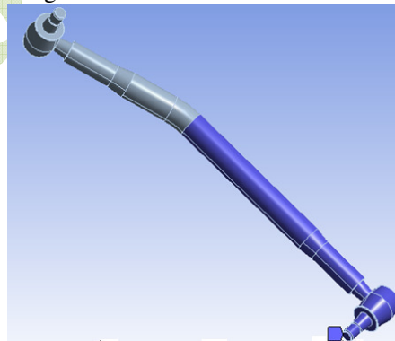
Fig.7 Fixed support
