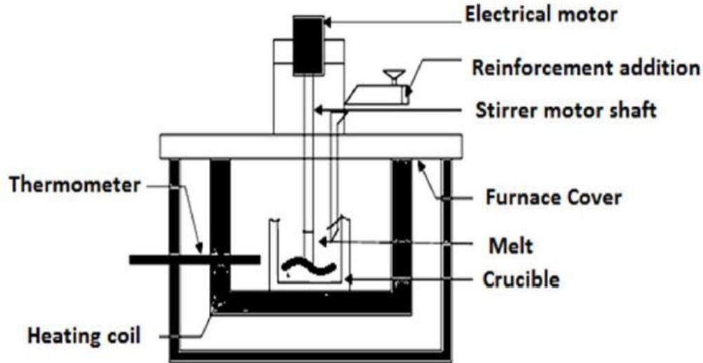
Fig 1 Schematic view of stir casting setup [7].
