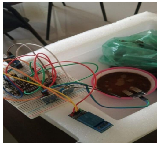
FIGURE 3. Relay connection to NodeMCU for smart farming.
