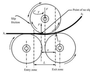
Fig 2. Shape rolling mechanism
