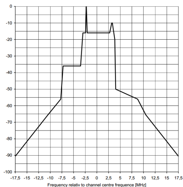
Gambar 9. Out-of-band spectrum mask TV analog 7 MHz (ETSI EN 302 297, 2005)
