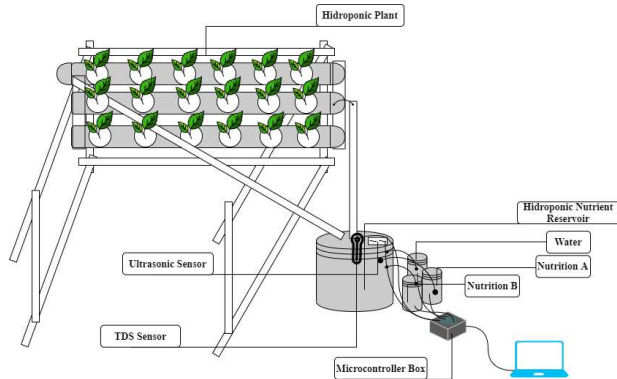
FIGURE 2. Hydroponic Control System Design
