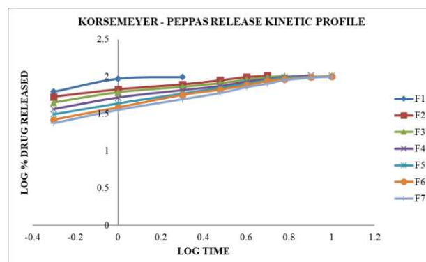
Figure 7: Korsemeyer – peppas release profile of different formulations
