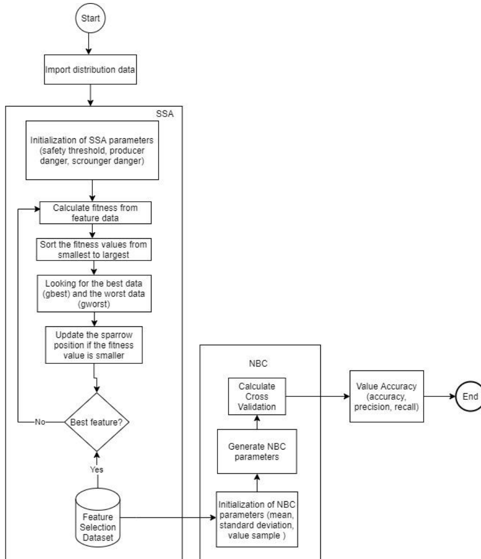
Figure 4. Training Model
