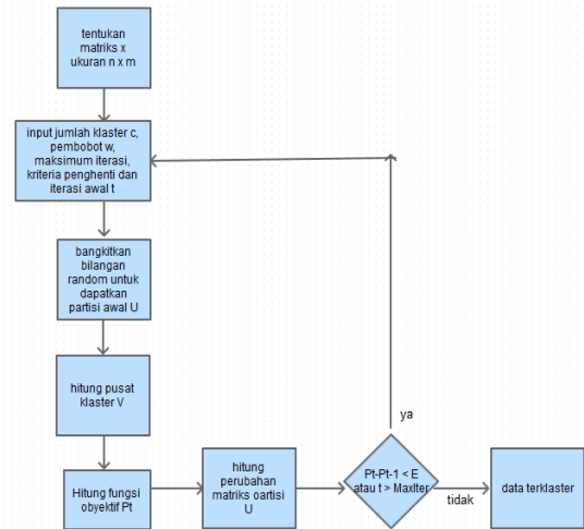
Gambar 4. Flowchart metode Fuzzy C Means
