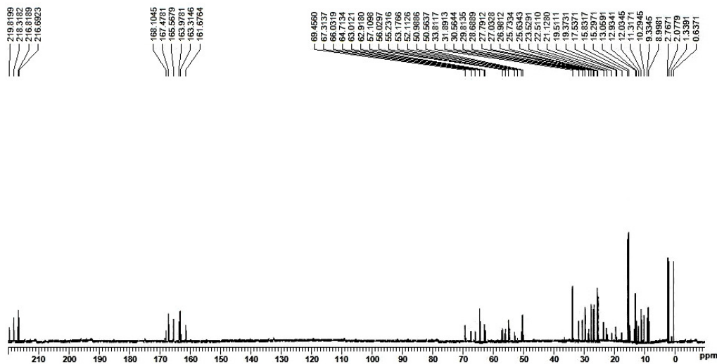
Fig. 5: 13 C spectrum of the purified bioactive 1-Monolinoleoylglycerol trimethylsilyl ether from seed of S. cumini
