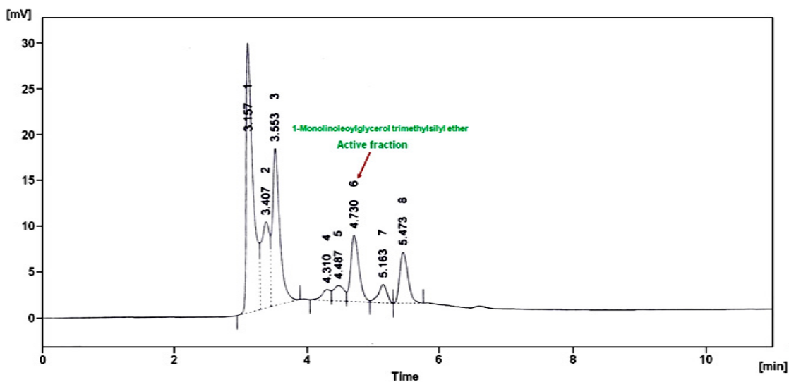
Fig. 2: HPLC chromatogram of the crude ethanol seed extract of S. cumini
