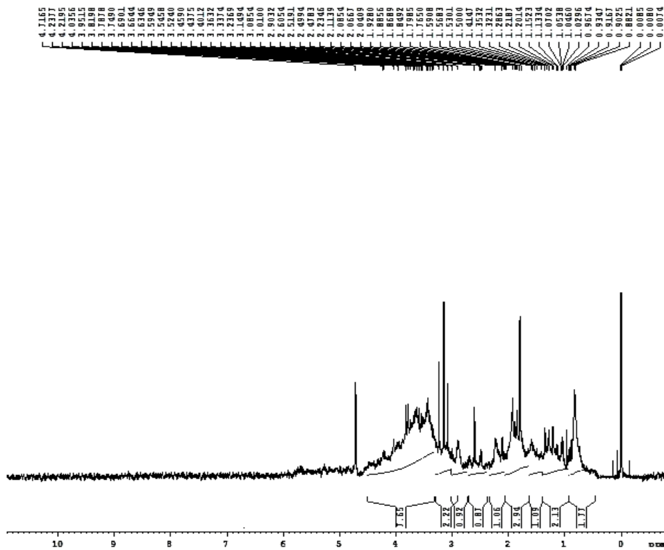
Fig. 4: 1 H spectrum of the purified bioactive 1-Monolinoleoylglycerol trimethylsilyl ether from seed of S. cumini
