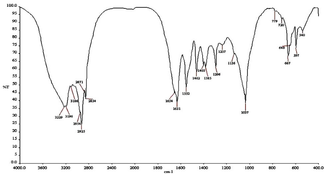
Fig. 3: FT-IR spectrum of the purified bioactive 1-Monolinoleoylglycerol trimethylsilyl ether from seed of S. cumini
