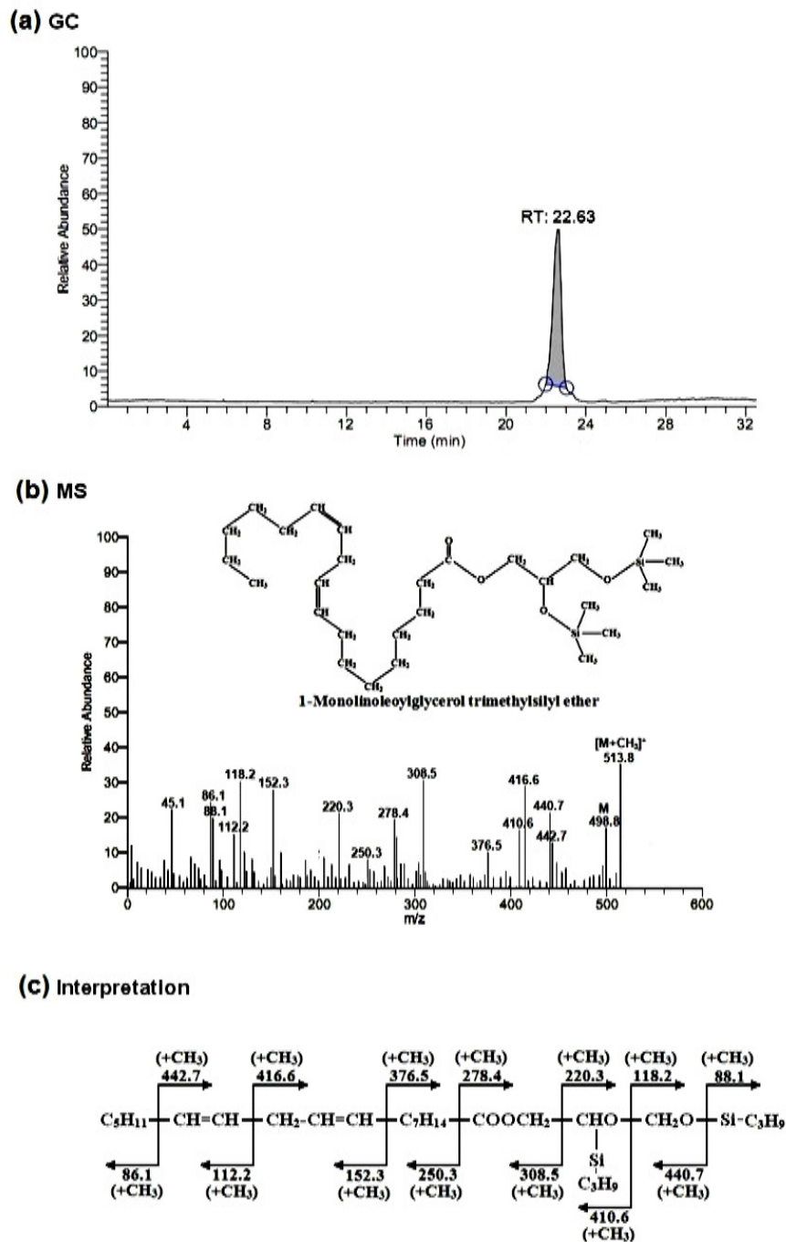
Fig. 6: (a) Gas Chromatography, (b) Mass spectrum and (C) molecular weight interpretations of the purified bioactive 1-Monolinoleoylglycerol trimethylsilyl ether from seed of S. cumini
