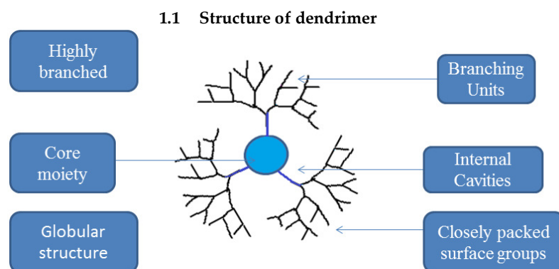
Fig.1 The structure of dendrimer.
