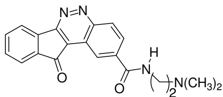
Figure.8: Indeno [1, 2-C]Cinnoline-11-one
