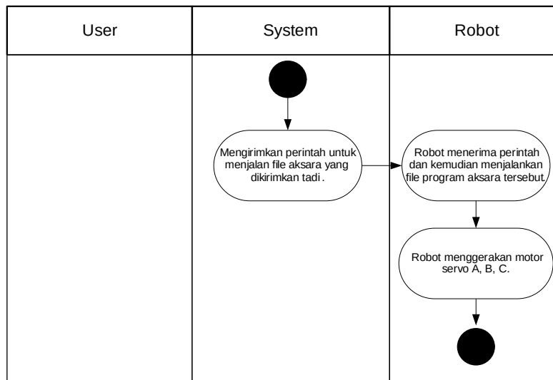
Gambar 3.4 Activity Diagram Proses Penulisan Karakter
