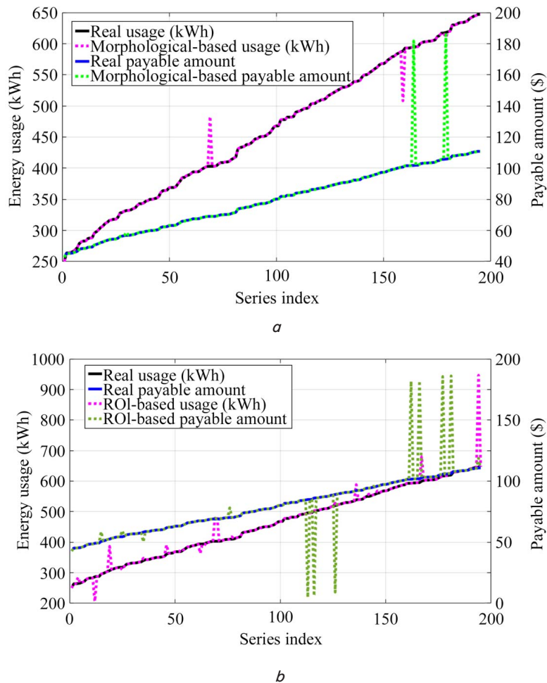
Fig. 8. The obtained texts of energy usage and payable amount of 195 bills are graphically expressed: a – comparison between the real and Morphological-based OCR; b – comparison between the real and ROI-based OCR
