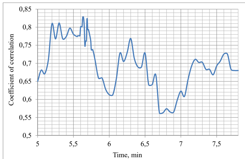
Fig. 6. Sliding control of the correlation coefficient
