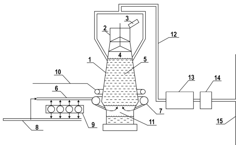
Fig. 1. Blast furnace and its blast path: 1 – furnace housing; 2 – charge material loader; 3 – skip; 4 – furnace top; 5 – column of charge materials; 6 – hot blast pipeline; 7 – ring pipeline; 8 – cold blast pipeline; 9 – air heaters; 10 – pipeline of fuel additives; 11 – furnace hearth; 12 – top gas flue; 13 – gas cleaning station; 14 – drop catcher; 15 – shop collector of blast-furnace gas
