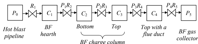
Fig. 9. A common channel for movement of gas flow in a blast furnace
