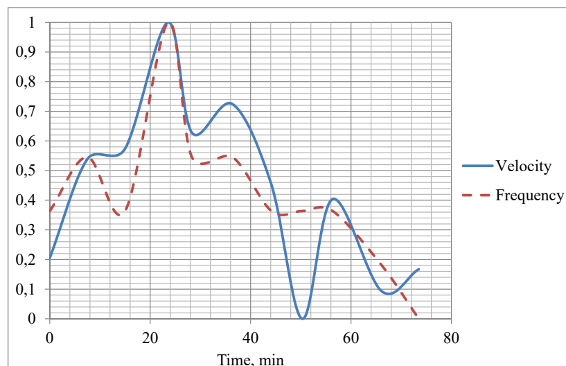
Fig. 7. Normalized curves of estimating the charge subsidence velocity and frequency of fluctuations of the lower pressure differential calculated with a discrete time of 5.63 min
