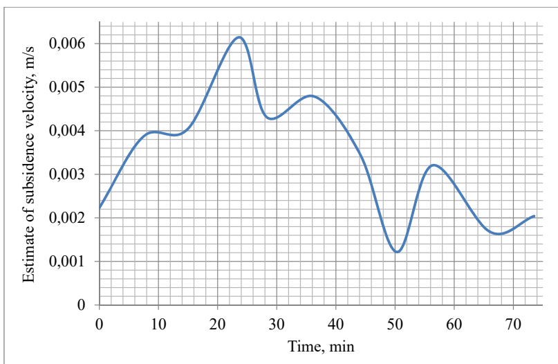
Fig. 4. Estimates of the charge subsidence velocity in one hour of blast furnace operation
