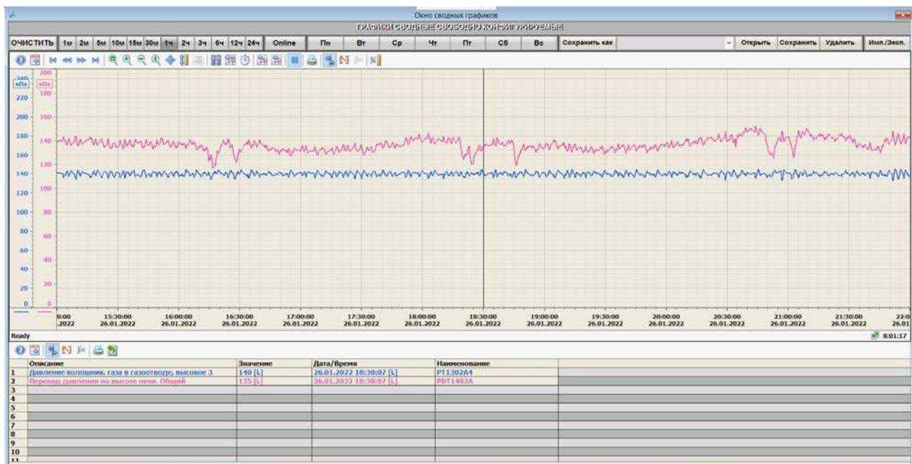
Fig. 2. Fluctuations in gas pressure at the top and the total pressure drop along the height of the furnace (the photo was taken from the SCADA system)
