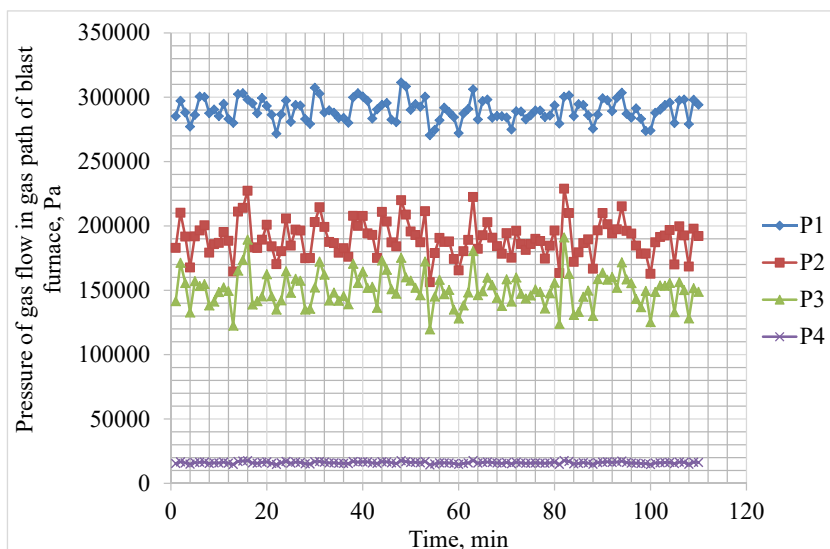
Fig. 10. Graphs of gas pressure fluctuations in the gas path of the blast furnace: P_1 – the gas pressure in the furnace hearth; P_2 – the gas pressure in the middle of the furnace shaft; P_3 – gas pressure at the top; P_4 – pressure downstream the droplet eliminator
