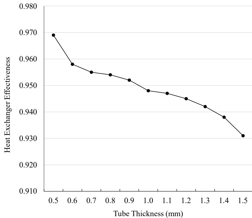
Fig. 3. Tube thickness vs heat exchanger effectiveness
