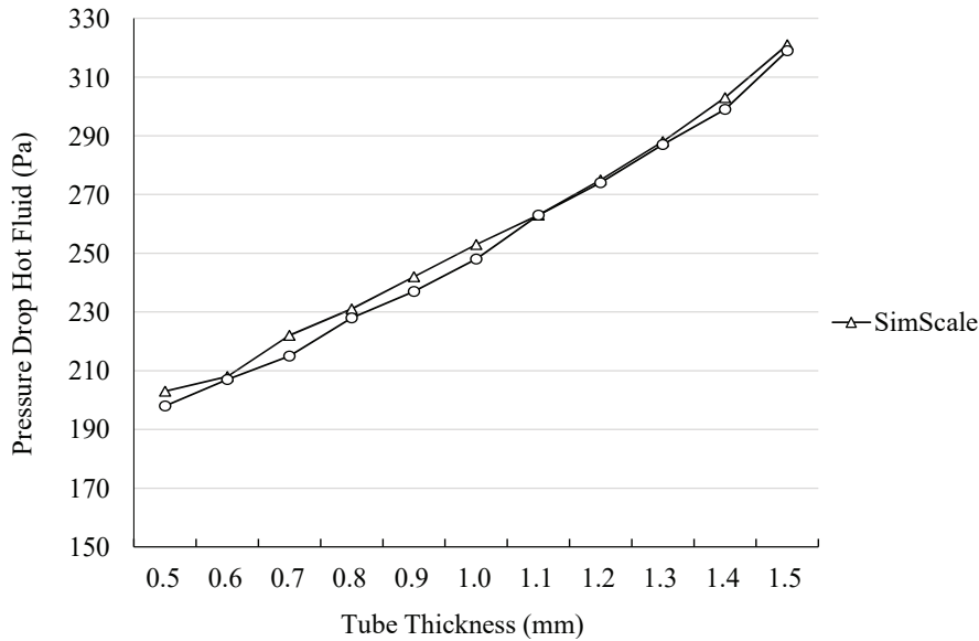
Fig. 6. Hot fluid pressure drop
