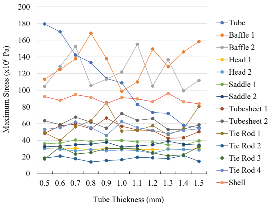
Fig. 9. Maximum stress on heat exchanger components
