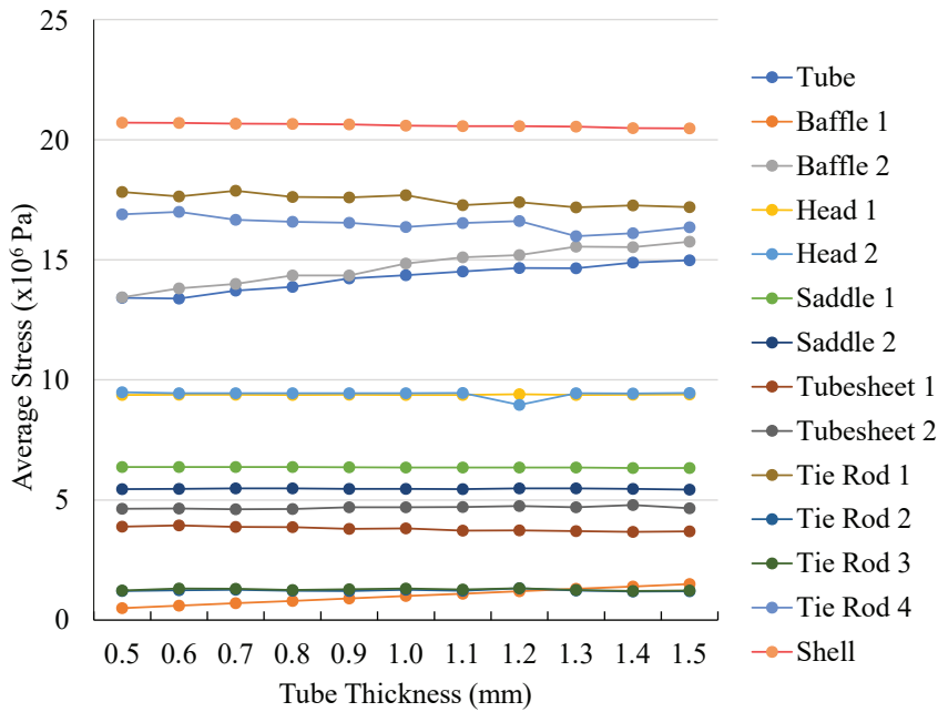
Fig. 10. Average stress on heat exchanger component
