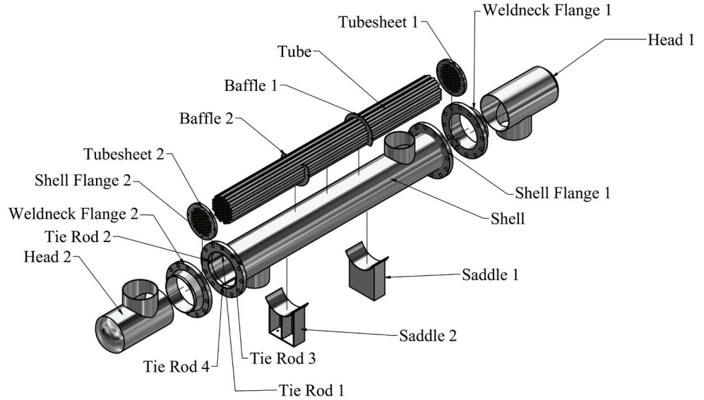
Fig. 1. Geometry of shell and tube heat exchanger
