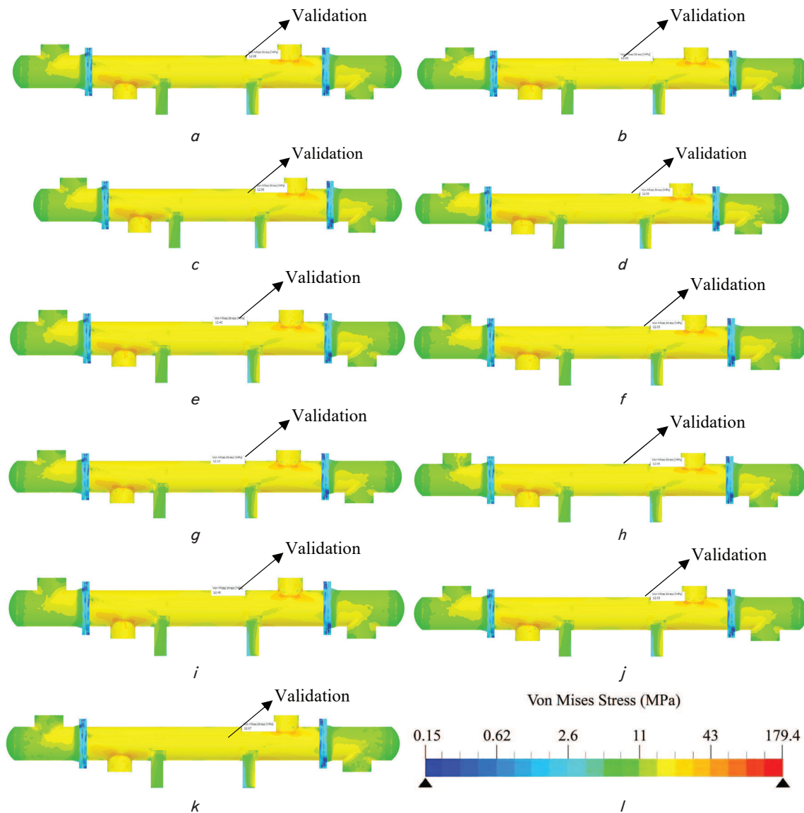
Fig. 7. Von Mises stress validation points by SimScale, tube thickness variations: a – 0.5 mm; b – 0.6 mm; c – 0.7 mm; d – 0.8 mm; e – 0.9 mm; f – 1.0 mm; g – 1.1 mm; h – 1.2 mm; i – 1.3 mm; j – 1.4 mm; k – 1.5 mm; l – Von Mises stress scale
