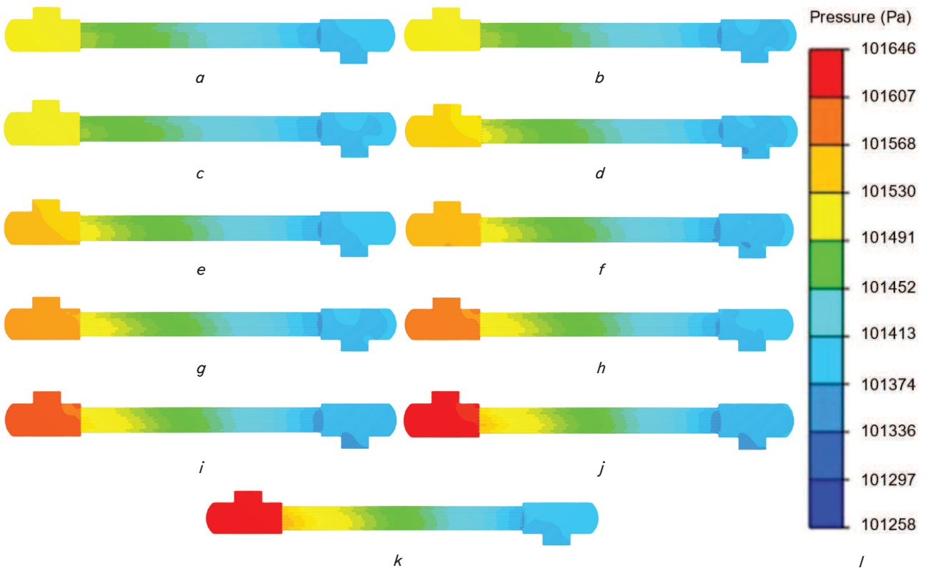
Fig. 5. Hot fluid pressure distribution, tube thickness variations: a – 0.5 mm; b – 0.6 mm; c – 0.7 mm; d – 0.8 mm; e – 0.9 mm; f – 1.0 mm; g – 1.1 mm; h – 1.2 mm; i – 1.3 mm; j – 1.4 mm; k – 1.5 mm; l – pressure scale
