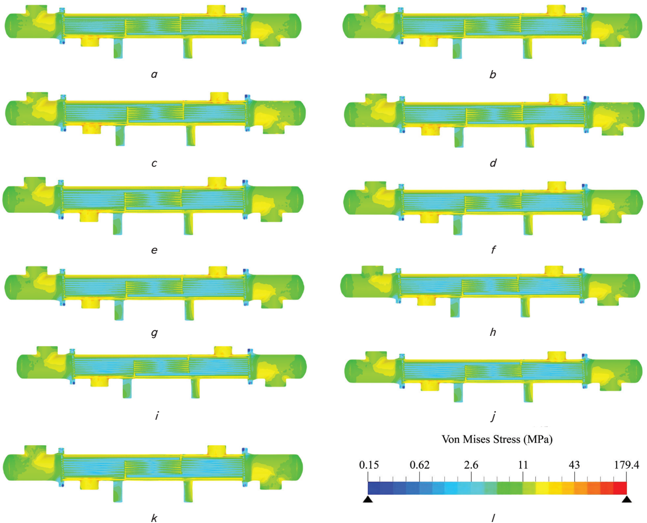
Fig. 8. Von Mises stress distribution on the section view of heat exchanger, tube thickness variations: a – 0.5 mm; b – 0.6 mm; c – 0.7 mm; d – 0.8 mm; e – 0.9 mm; f – 1.0 mm; g – 1.1 mm; h – 1.2 mm; i – 1.3 mm; j – 1.4 mm; k – 1.5 mm; l – Von Mises stress scale
