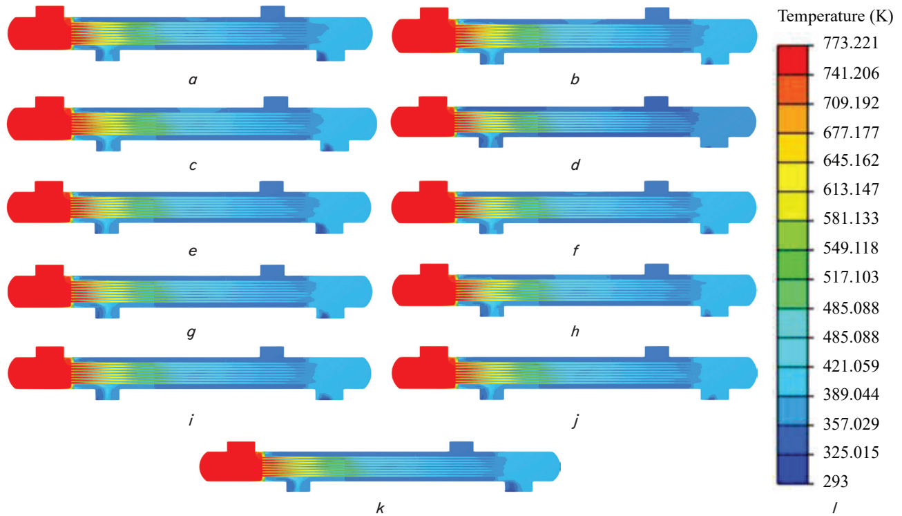
Fig. 2. Temperature distribution of simulation, tube thickness variations: a – 0.5 mm; b – 0.6 mm; c – 0.7 mm; d – 0.8 mm; e – 0.9 mm; f – 1.0 mm; g – 1.1 mm; h – 1.2 mm; i – 1.3 mm; j – 1.4 mm; k – 1.5 mm; l – temperature scale
