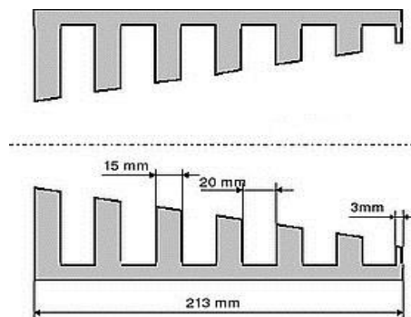
Figure 1. PTB collimator design is according to ISO 4037-1.
