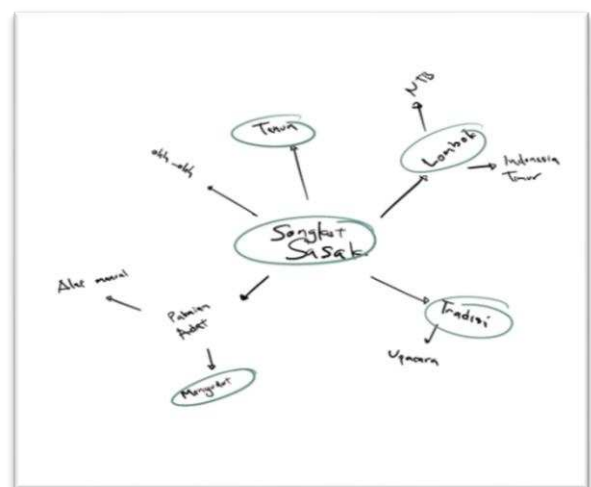
Gambar 1. Mind Mapping
