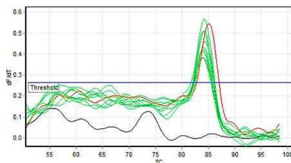
Figure 1. Melt curve analysis for T m . Green: samples; Red: positive control; Black: negative control
