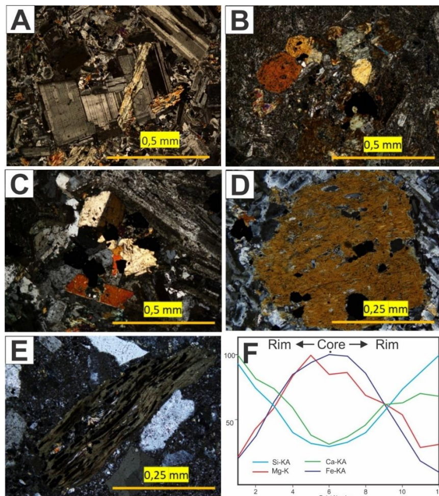
Figure 7. Photomicrograph of alkali feldspar and pyroxene in Raya Volcanic samples. (A) Alkali Feldspar, (B) twin pyroxene, (C) glomerocryst-pyroxene and plagioclase, (D) opaque inclusion in pyroxene, (E) opacitization in pyroxene, and (F) normal zoning pattern of pyroxene phenocryst.
