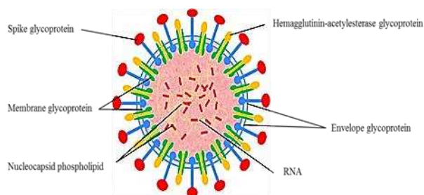
Figure 4. Schematic diagram of coronavirus present different membrane proteins
