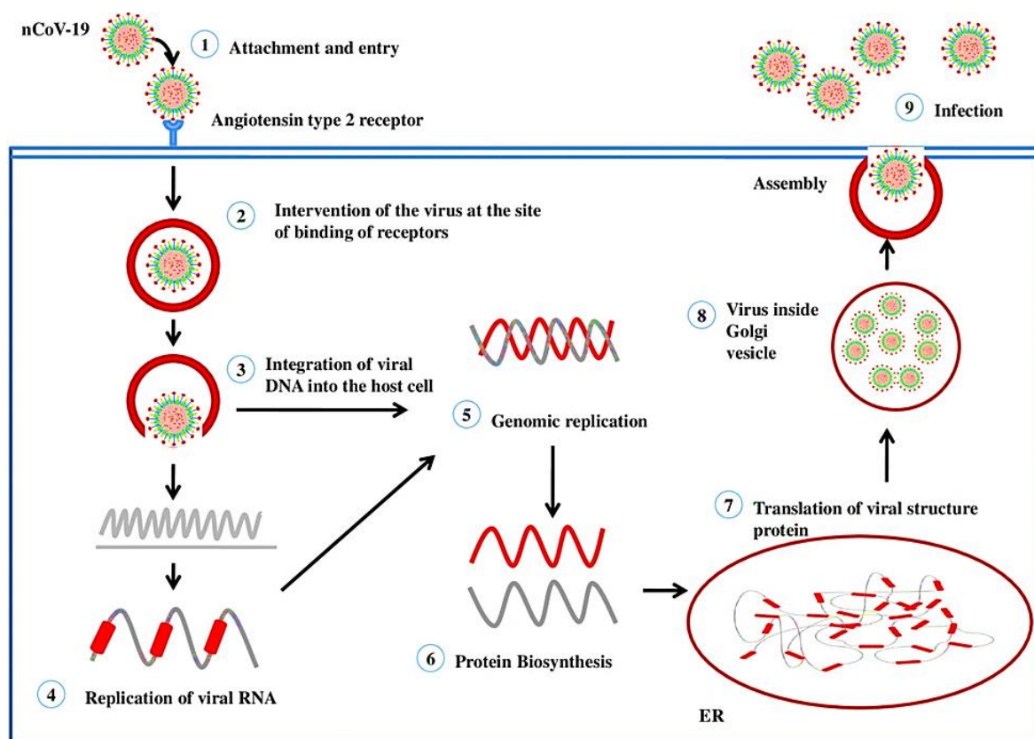
Figure 5. Replication process of SARS-CoV-2
