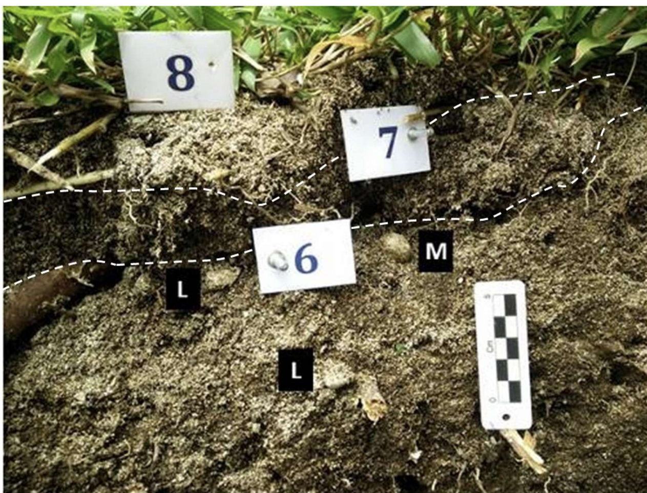
Figure 3. A 2006 tsunami deposit layer in Pangandaran, characterized by light brown color with still-intact mollusc clasts of Neritina sp. (M) and lithic fragments (L). The top of deposit layer is marked with number 7 label. Scale bar = 5 cm.
