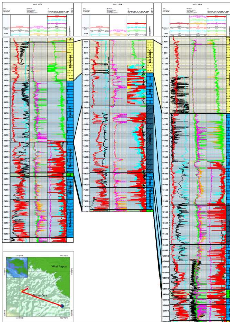
Figure 5. Well logs correlation of three wells on Berau Basin
