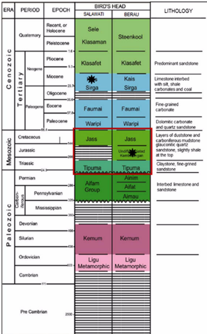
Figure 3. Regional stratigraphy of West Papua waters (modified after Sapiie et al. , 2012)
