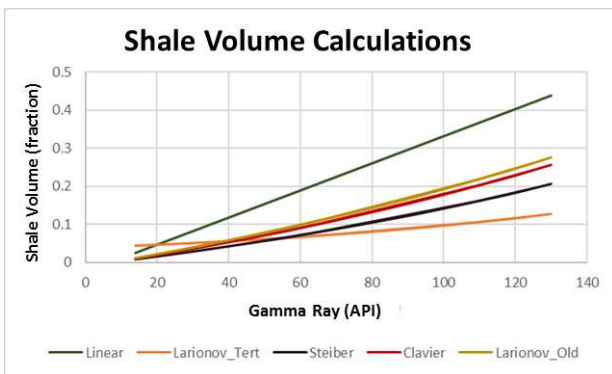
Figure 8. Comparison graph of linear and non-linear shale volume calculations
