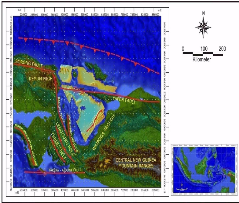
Figure 1. West Papua Bird's Head tectonic elements (Adyagharini, 2009)
