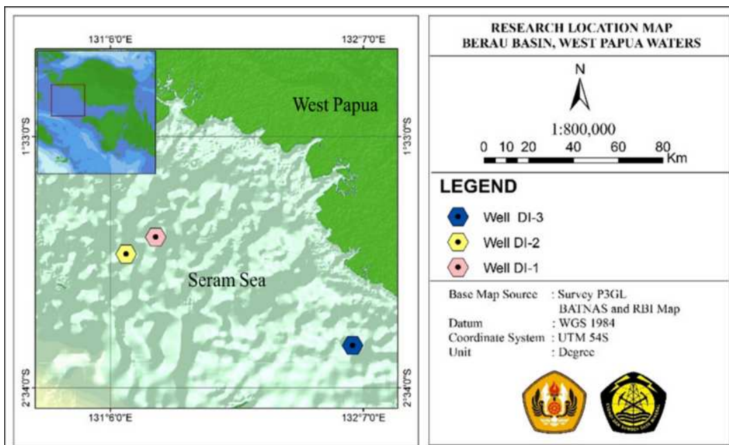
Figure 4. Map of research location, West Papua Waters
