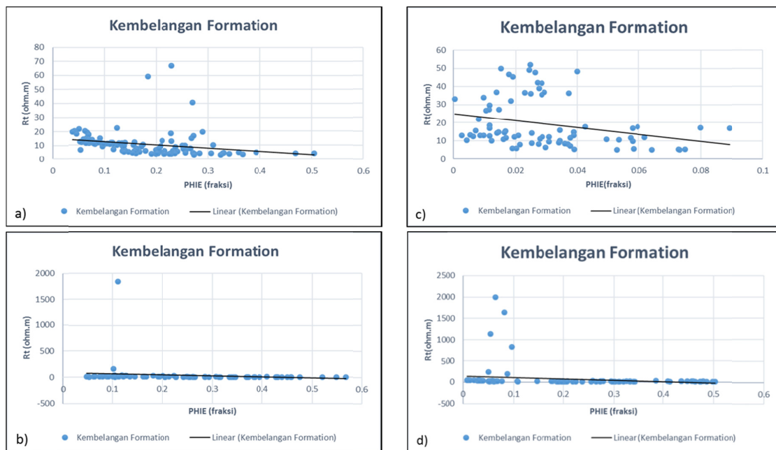
Figure 9. PHIE to R_t plot of 2 zones in Kembelangan Formation
