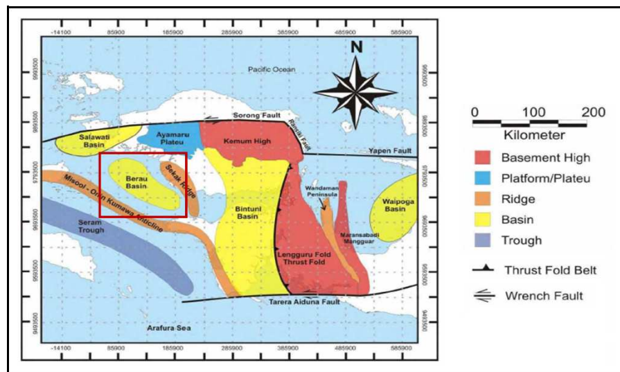
Figure 2. West Papua Bird's Head tectonic elements (Pigram et al. , 1982)
