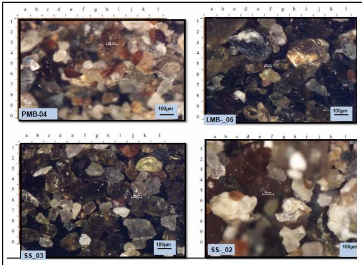
Figure 5. Mineralogical analysis: Sample PMB-04 shows coarse sand sediment. diagenetic features of fragmentation, followed by ferro nickel (kj 3-4), magnetic (bc 4-6), and plagioclase (jk,4-5). Sample LMB-06 demonstrates coarse sand unit with fragments of covalite (gj, 3-5), nickel-iron (hj 1-2), serpentinic rock (ac6-9) and feldspar (fg2-3). Sample SS-03 shows coarse sand. Sample SS-02 exhibits coarse sand with ferro nickel (be,1-5), magnesit (ac,6-8), and magnetic (ik,8-9).
