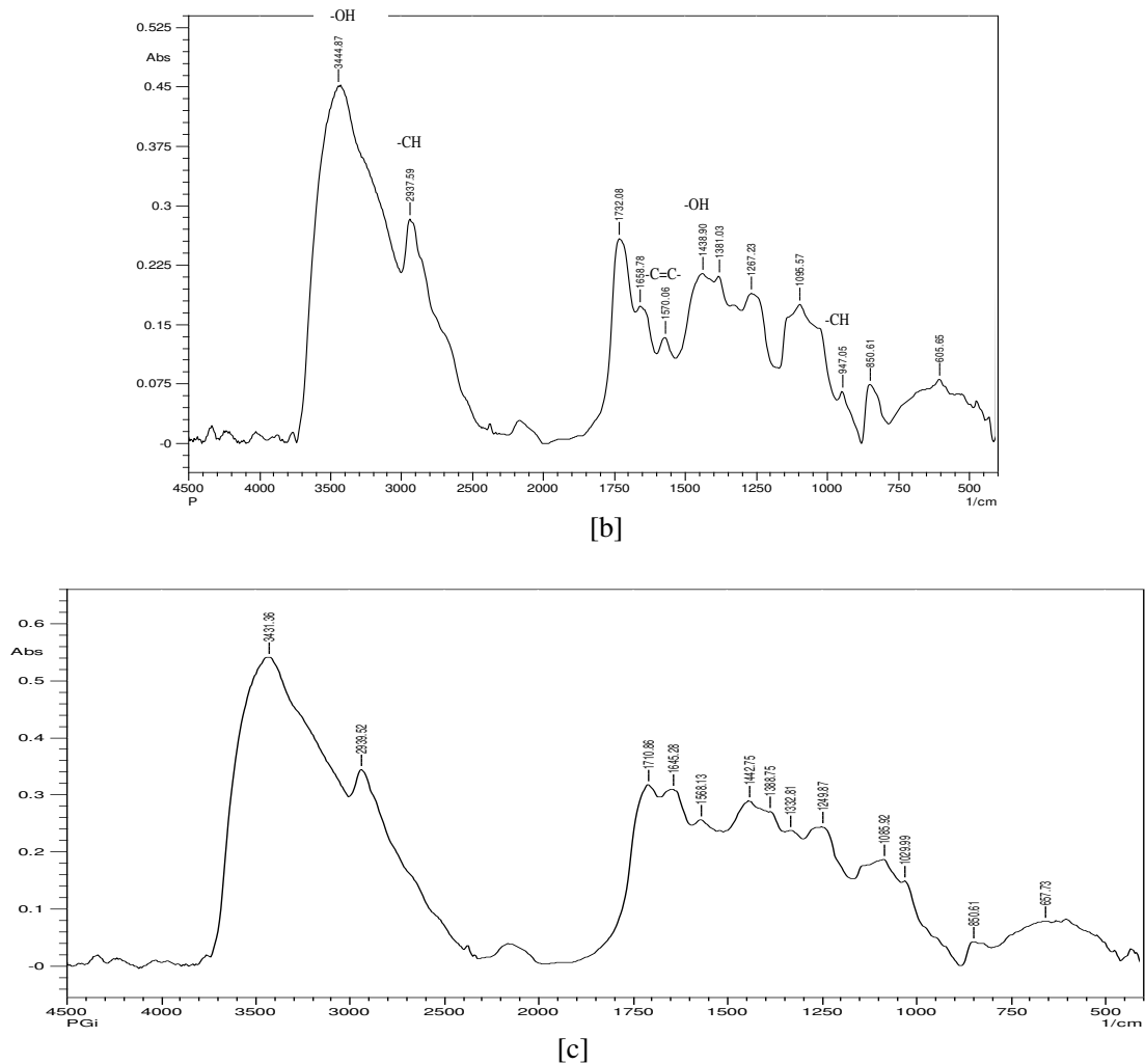
Gambar 7. Spektra FTIR [a] gelatin, [b] PVA, [c] PVA/gelatin
