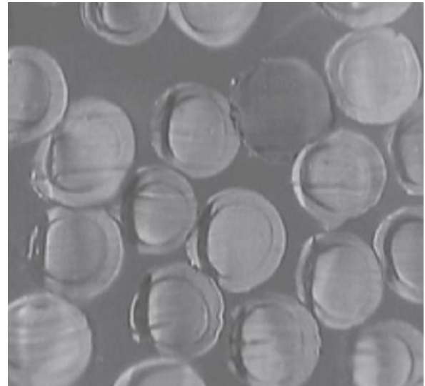
Gambar 4. Penampang melintang poliester low melt fiber 16
