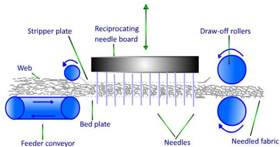
Gambar 3. Diagram proses needle punch 13
