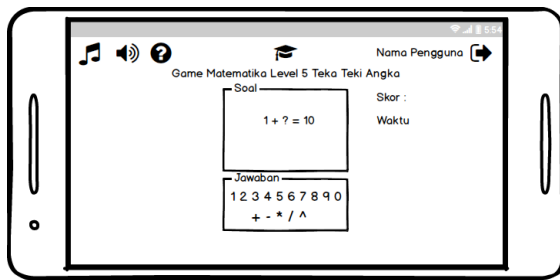
Gambar 11 Game Level 4
