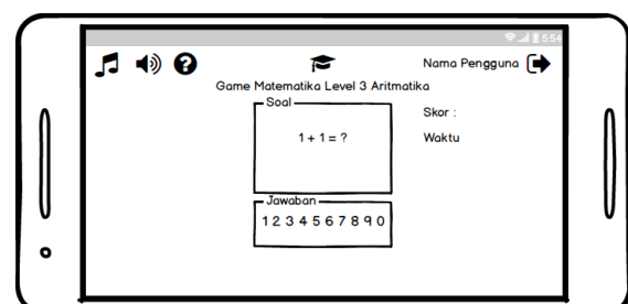
Gambar 10 Game Level 3
