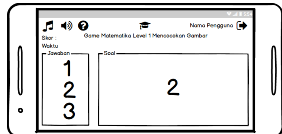
Gambar 8 Game Level 1
