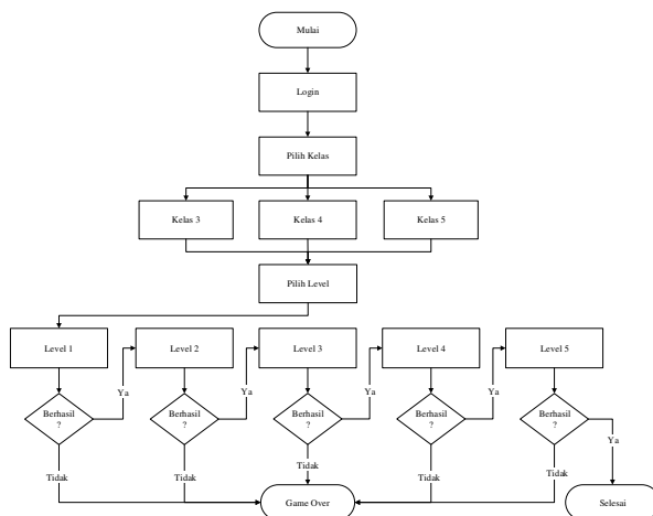
Gambar 2 Flowchart System
