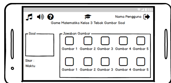
Gambar 9 Game Level 2
