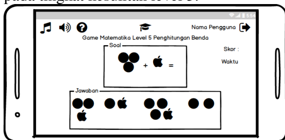
Gambar 12 Game Level 5
