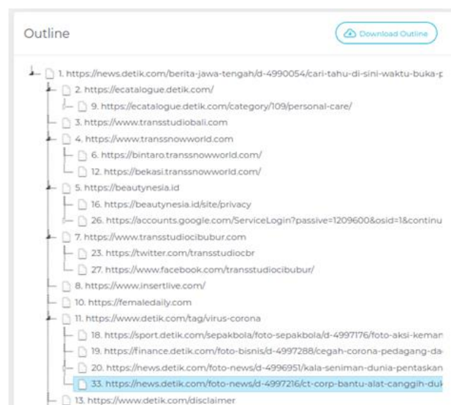
Gambar. 5. Outline Tree
