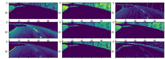
Gambar. 3. Output Convolutional0
