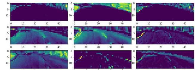
Gambar. 4. Output Convolutional1
