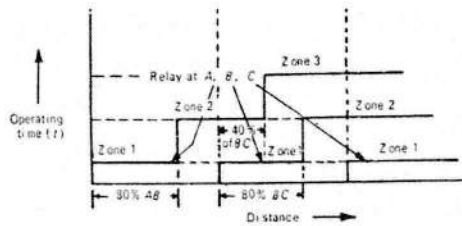
Gambar 5. Metode definitif-time .
