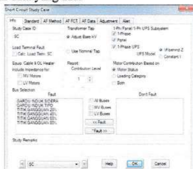
Gambar 12. Data Short Circuit Study Case Pada Software ETAP ( Electric Transient and Analysis Program ) 12.6.0.
