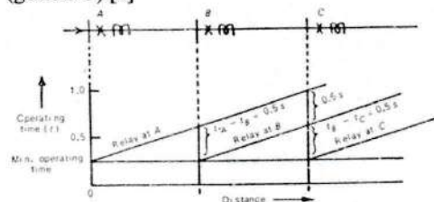
Gambar 4. Metode distance-time .
