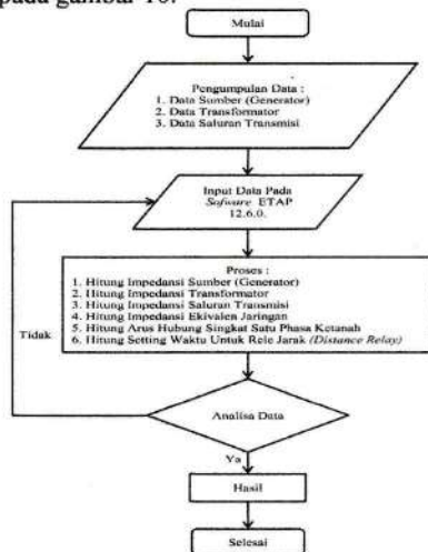
Gambar 10. Diagram Alir (flowchart).
