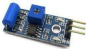
Gambar 2.6: Sensor getar SW-420 (Najmurrokhman, 2018)
