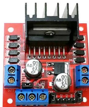
Gambar 10. Driver motor L298N (Sumber: www.nyebarilmu.com , 2020)
