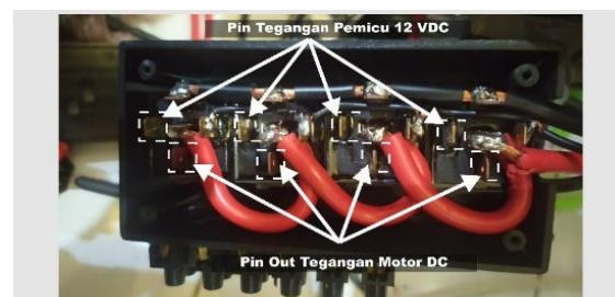
Gambar 8. Rangkaian relay 5K 12 VDC 40A
