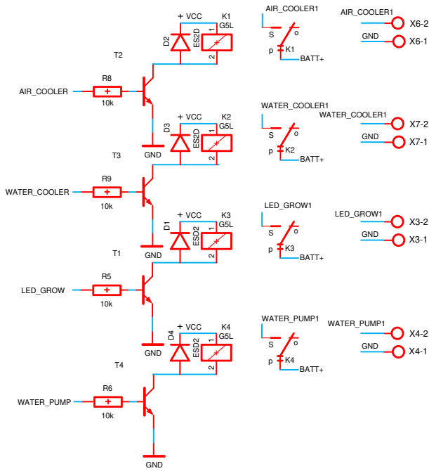
Figure 5. Relay circuit
