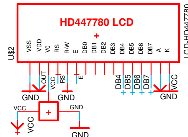
Figure 8. LCD circuit
