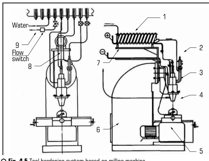
○ Fig. 4.5 Tool hardening system based on milling machine
