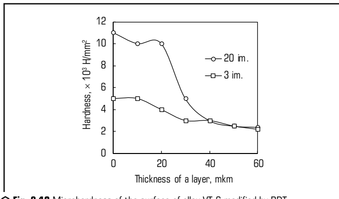
○ Fig. 8.19 Microhardness of the surface of alloy VT-6 modified by PDT
