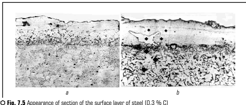
○ Fig. 7.5 Appearance of section of the surface layer of steel (0.3 % C) after one-pulse microsurfacing: a – with titanium; b – with tungsten
