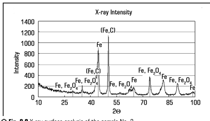
○ Fig. 8.9 X-ray surface analysis of the sample No. 3
