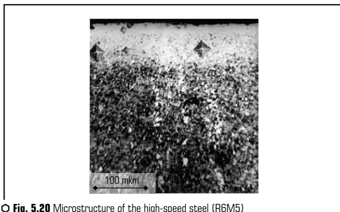
○ Fig. 5.20 Microstructure of the high-speed steel (R6M5) layer hardened by PDT (molybdenum electrode, 6 pulses)
