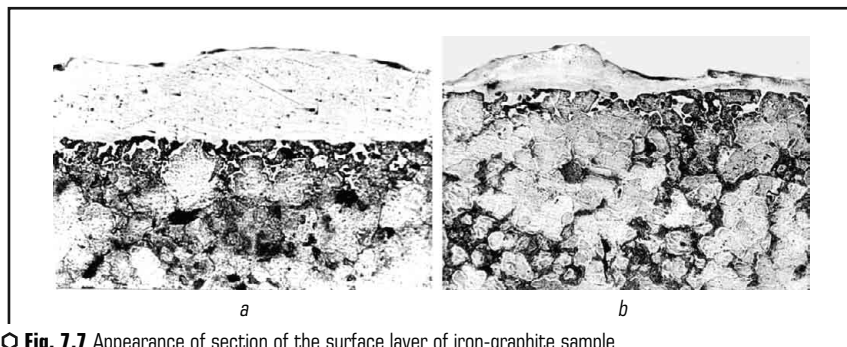
○ Fig. 7.7 Appearance of section of the surface layer of iron-graphite sample after treatment with one plasma pulse containing: a – titanium; b – tungsten
