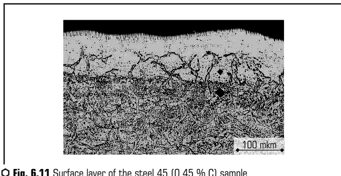
○ Fig. 6.11 Surface layer of the steel 45 (0.45 % C) sample after PDT (5 pulses)
