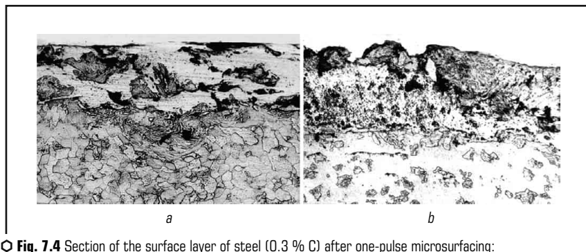
Fig. 7.4 Section of the surface layer of steel (0.3 % C) after one-pulse microsurfacing: a – with copper; b – with aluminium
