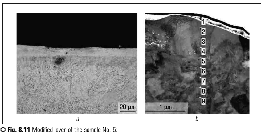
○ Fig. 8.11 Modified layer of the sample No. 5:
