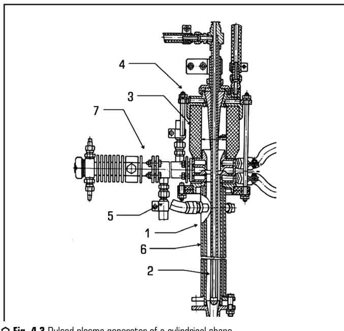
○ Fig. 4.3 Pulsed plasma generator of a cylindrical shape
