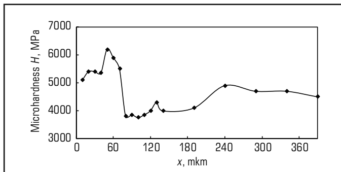
○ Fig. 9.3 Changing the nature of the distribution of integral microhardness from the outer surface to be treated to the base metal
