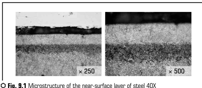
○ Fig. 9.1 Microstructure of the near-surface layer of steel 40X during pulsed plasma treatment
