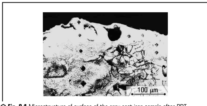
○ Fig. 8.1 Microstructure of surface of the grey cast iron sample after PDT
