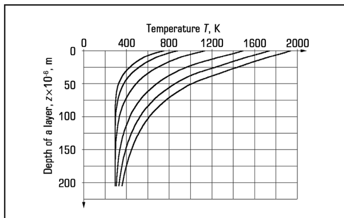
○ Fig. 6.2 Distribution of temperature through thickness of the surface layer at certain time moments t of heating: 1 – t = 4.5 \cdot 10^{-5} s; 2 – t = 7.5 \cdot 10^{-5} s; 3 – t = 1.5 \cdot 10^{-4} s; 4 – t = 3.0 \cdot 10^{-4} s; 5 – t = 4.5 \cdot 10^{-4} s; 6 – t = 6.0 \cdot 10^{-4} s
