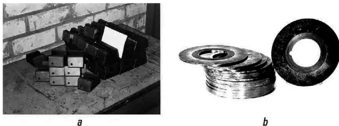
○ Fig. 10.1 Hardened knives for cutting rolled stock: a – steel sheets; b – sections
