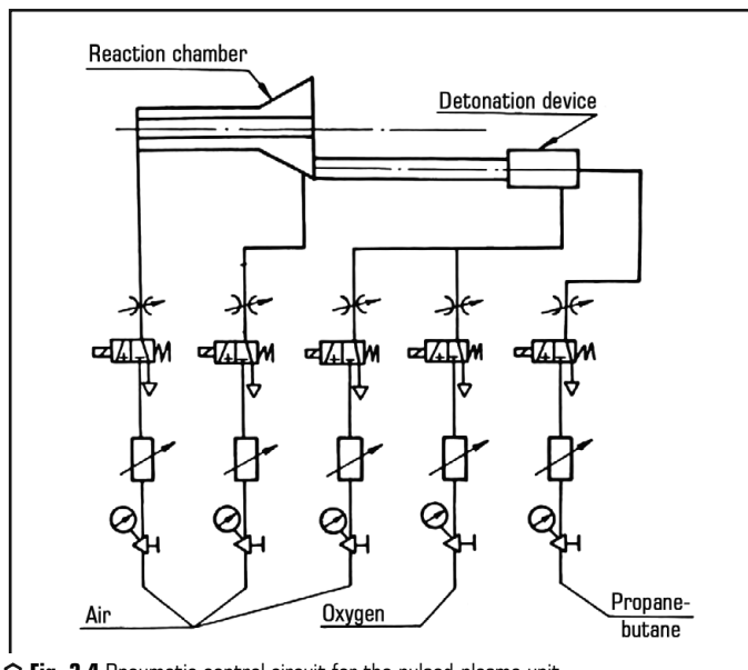
○ Fig. 3.4 Pneumatic control circuit for the pulsed-plasma unit
