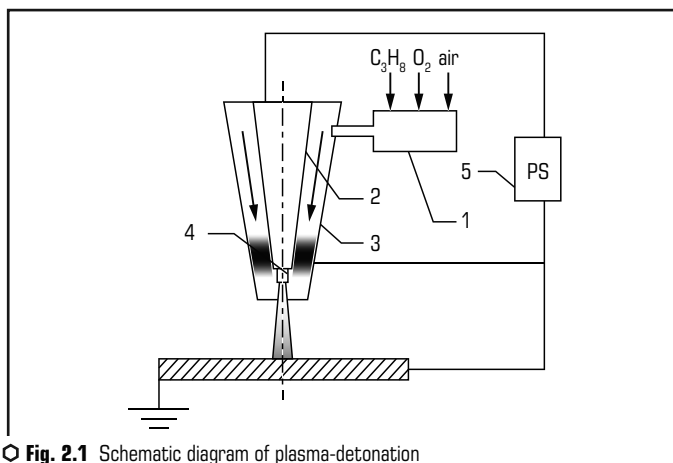
○ Fig. 2.1 Schematic diagram of plasma-detonation device – plasma generator
