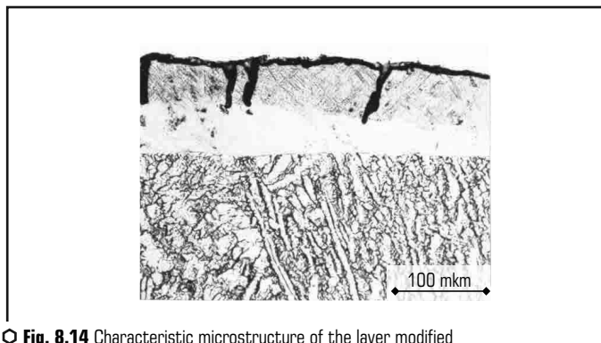
○ Fig. 8.14 Characteristic microstructure of the layer modified by PDT (single-pulse treatment) on the surface of alloy VT-22
