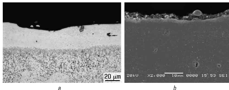
Fig. 8.8 Modified layer of the sample No. 3:
