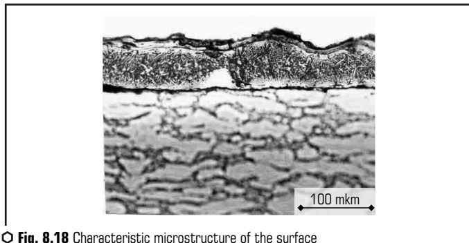
○ Fig. 8.18 Characteristic microstructure of the surface of alloy VT-6 modified by PDT with 20 pulses in nitrogen atmosphere
