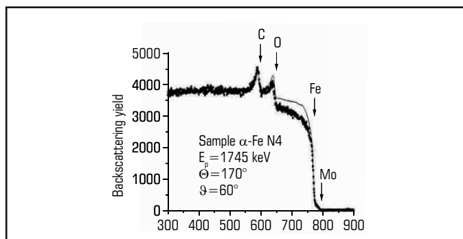
○ Fig. 6.9 Energy spectrum of Rutherford ion backscattering recorded by the method of elastic resonance of protons with an energy of 1.745 MeV to determine the concentration of carbon and oxygen on the \alpha -Fe sample after PDT (20 pulses)
