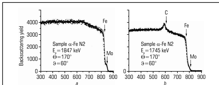
○ Fig. 6.8 Energy spectrum of Rutherford ion backscattering for the \alpha -Fe sample after PDT (10 pulses) recorded by using ^4\text{He} : a – determination of molybdenum concentration; b – determination of carbon
