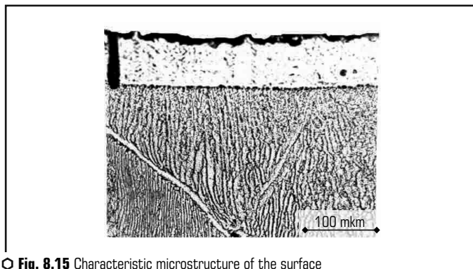
○ Fig. 8.15 Characteristic microstructure of the surface of alloy VT-22 modified by PDT (treatment with three pulses)
