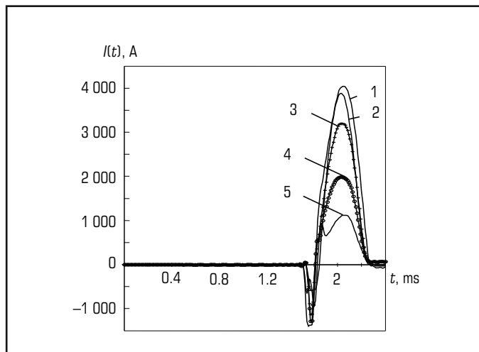
○ Fig. 3.13 Time diagram of electric current I (A) flowing between the consumable electrode tip and workpiece surface: 1 – h=20 mm, H=40 mm; 2 – h=0 mm, H=70 mm; 3 – h=20 mm, H=70 mm; 4 – h=40 mm, H=70 mm; 5 – h=20 mm, H=100 mm
