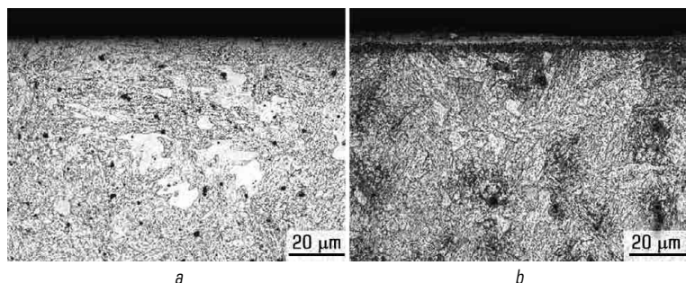
○ Fig. 8.7 Microsections of samples: a – No. 1; b – No. 2
