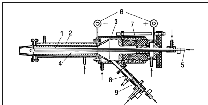
○ Fig. 3.2 Schematic of design of cylindrical pulsed plasma generator
