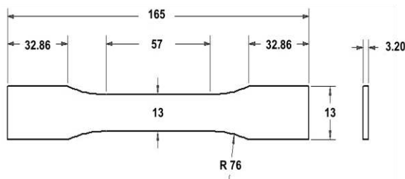
Figure 4. ASTM D638 type 1 tensile test specimen CAD design [12]
