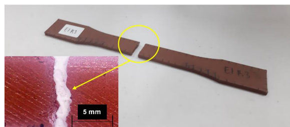
Figure 8. The fracture shape of the tensile test specimen
