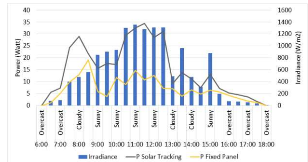
Figure 8. The comparison of generated power on March 28th 2021
