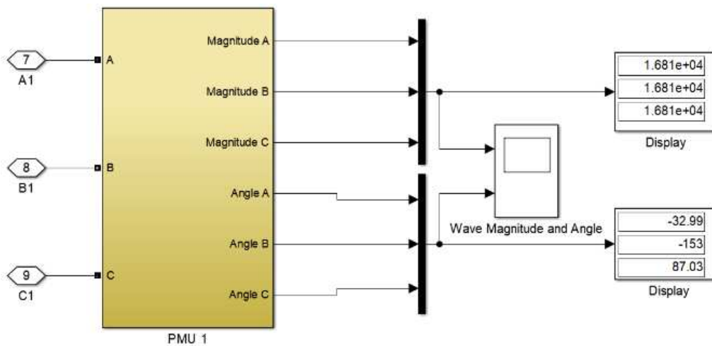
Figure 6. PMU module via Matlab/Simulink
