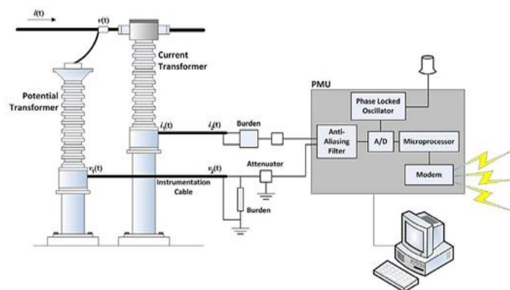
Figure 2. Schematic of a PMU connected to the power grid [19]
