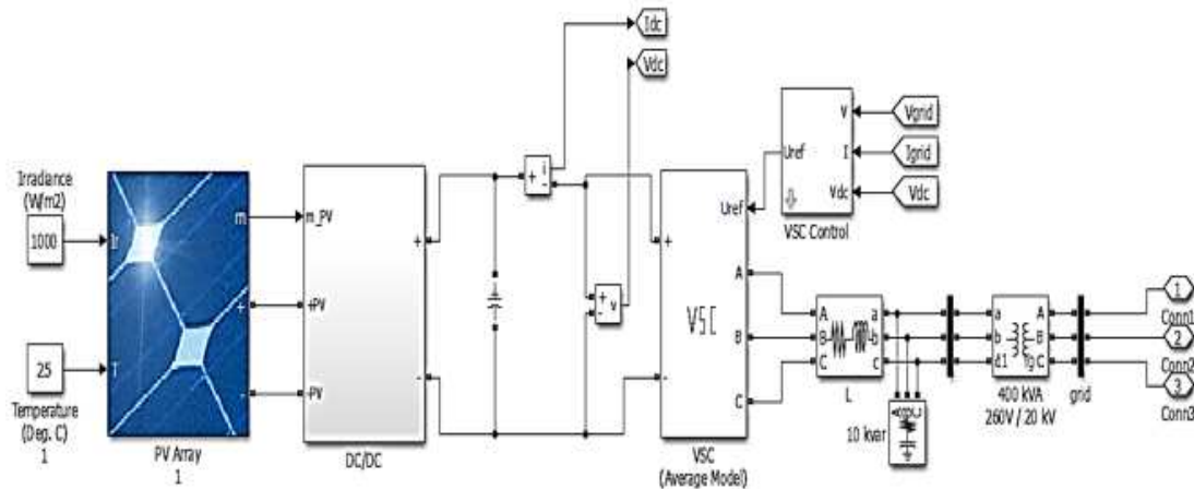
Figure 1. DG solar cell equalised by Matlab/Simulink
