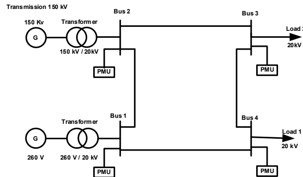
Figure 3. Single Line connected DG.
