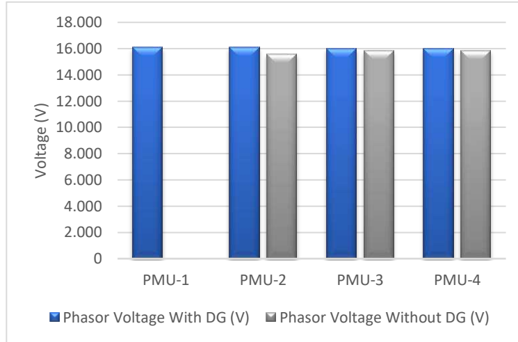
Figure 8. Comparison of the phasor voltages' positive sequence before and after DG
