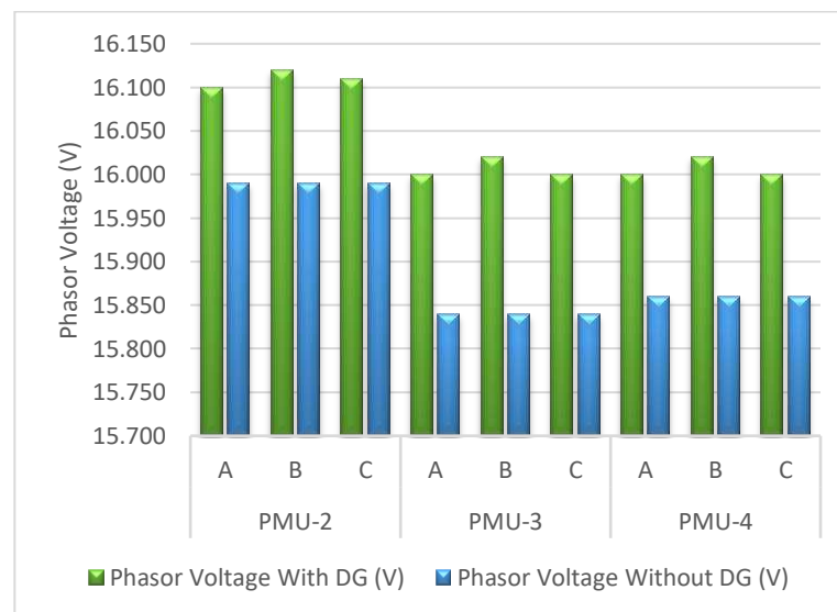
Figure 7. Comparison of phasor voltages before and after DG
