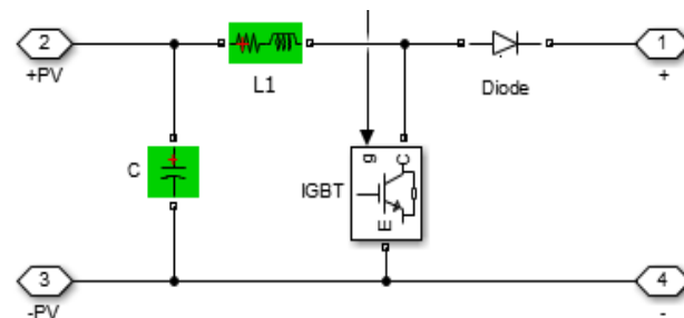
Figure 4. Boost Converter Topology
