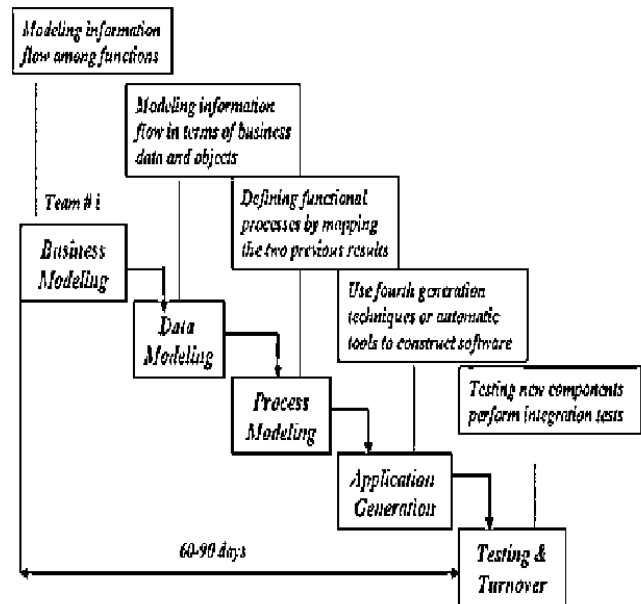
Gambar. 1. Model Rapid Application Development [7] [8]
