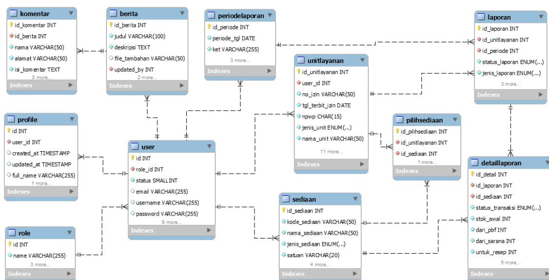
Gambar. 7. Physical Entity Relationship Diagram
