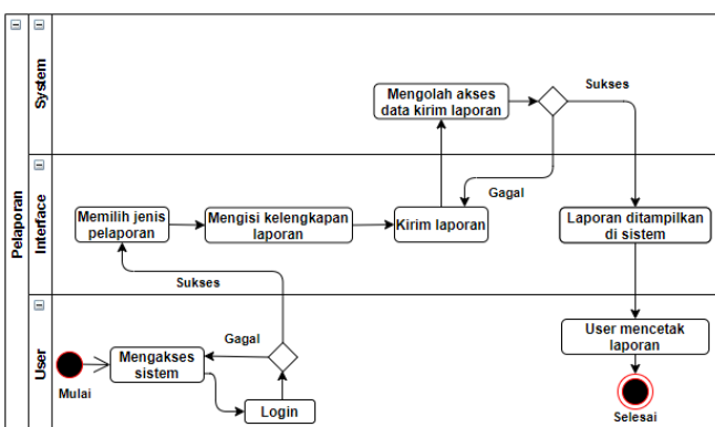
Gambar. 4. Activity Diagram Pelaporan
