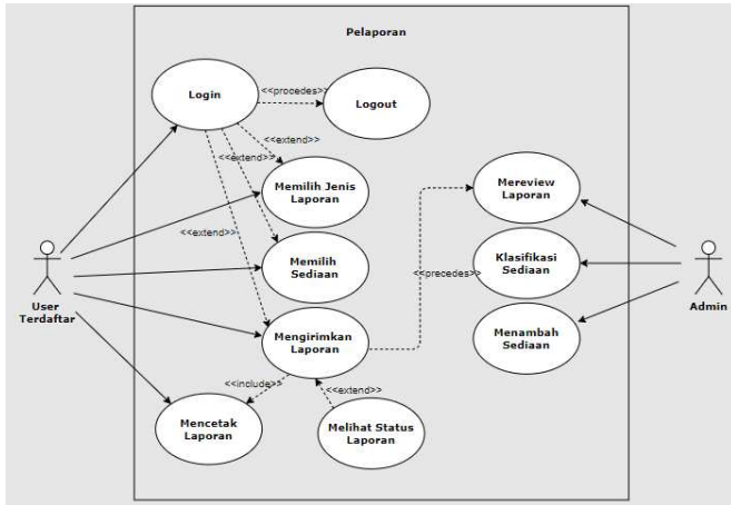
Gambar. 6. Use case Diagram Fungsi Pelaporan
