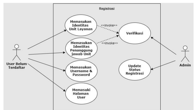
Gambar. 5. Use case Diagram Fungsi Registrasi
