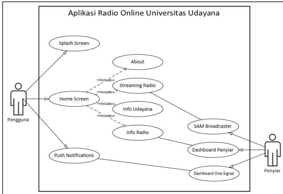
Figure 3. Use Case Diagram Aplikasi
