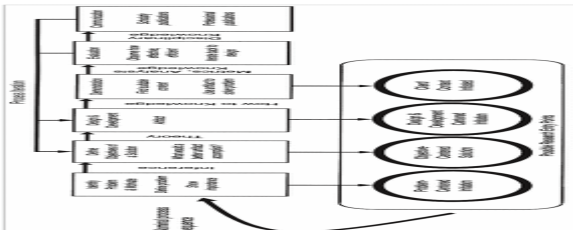
Figure 1. Metodologi DSRM
