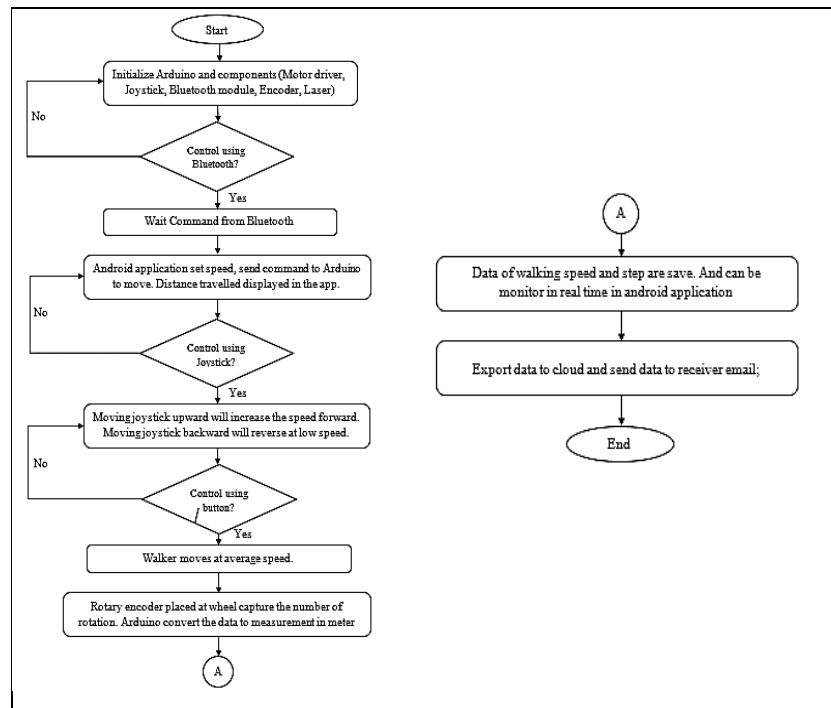
Figure 7. Flow chart of product
