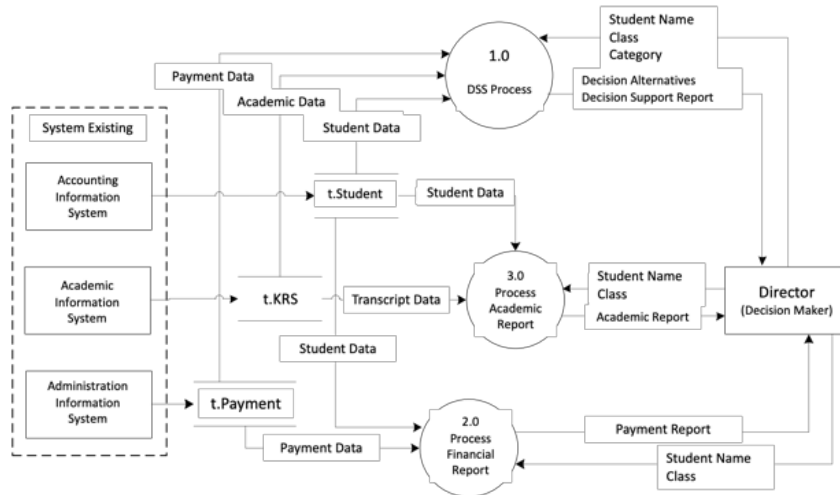
Fig. 5 – DFD Level 1 from Level 0 of DSS.
