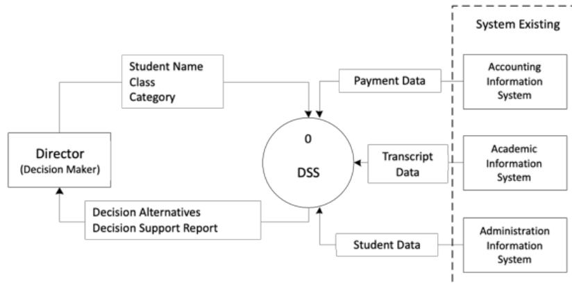
Fig. 4 – Context Diagram DSS-XYZ Midwifery Academy.
