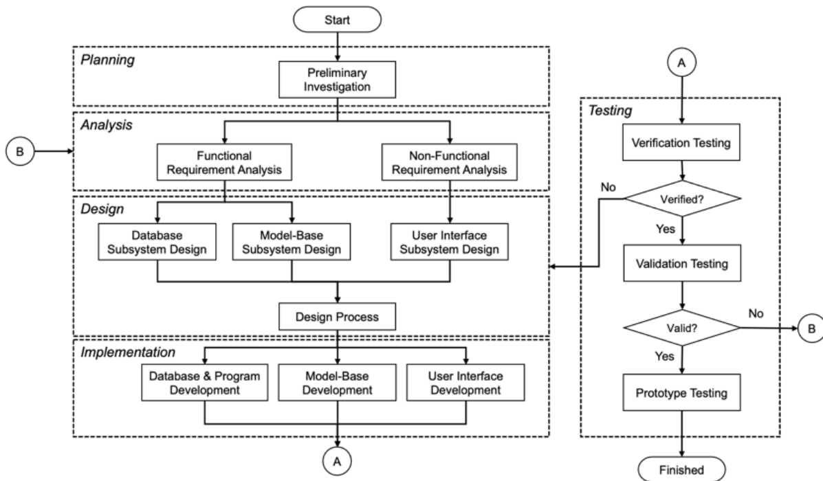
Fig. 2 – DSS development framework
