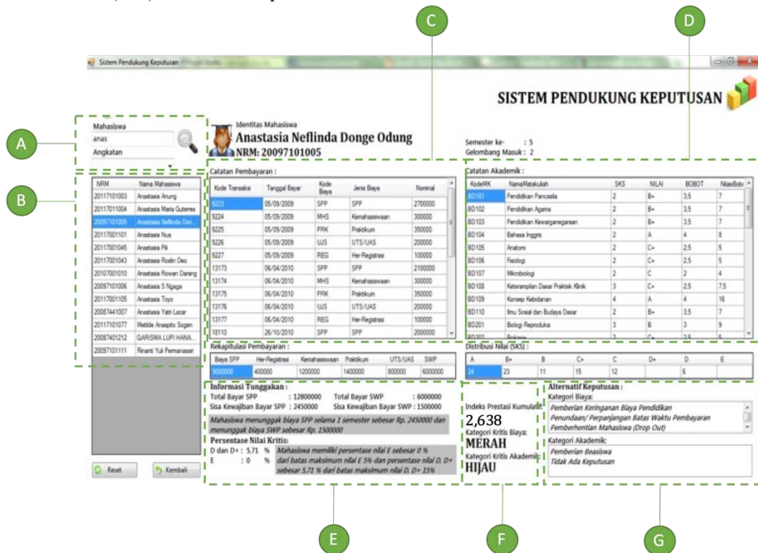
Fig. 9 – Display of the main DSS form.
