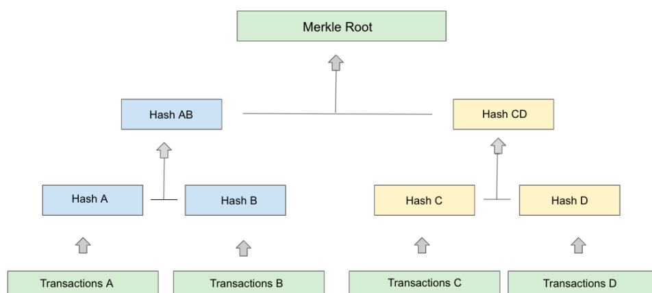
Figure 2. Merkle tree for 4 Hash codes
