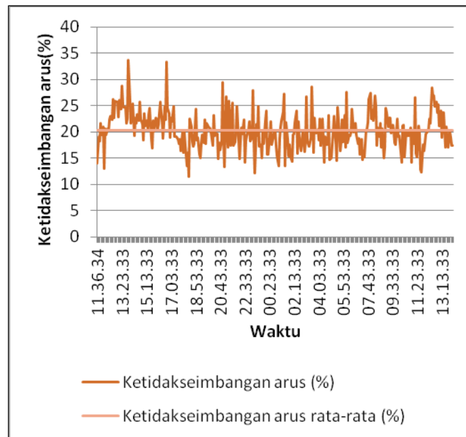
Figure 4. Graph of current imbalance between phases
