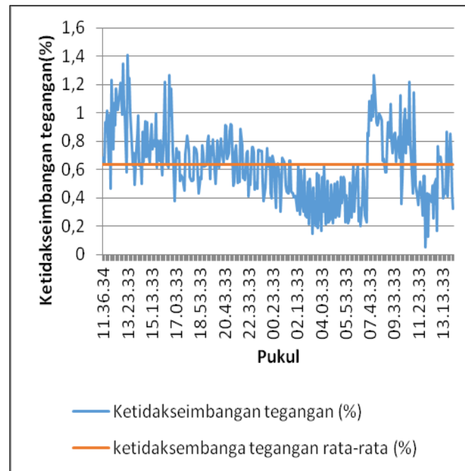
Figure 3. Graph of voltage imbalance between phases
