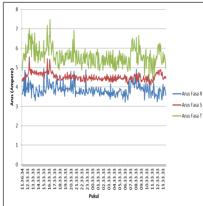
Figure1. Graph of current measurement data per phase
