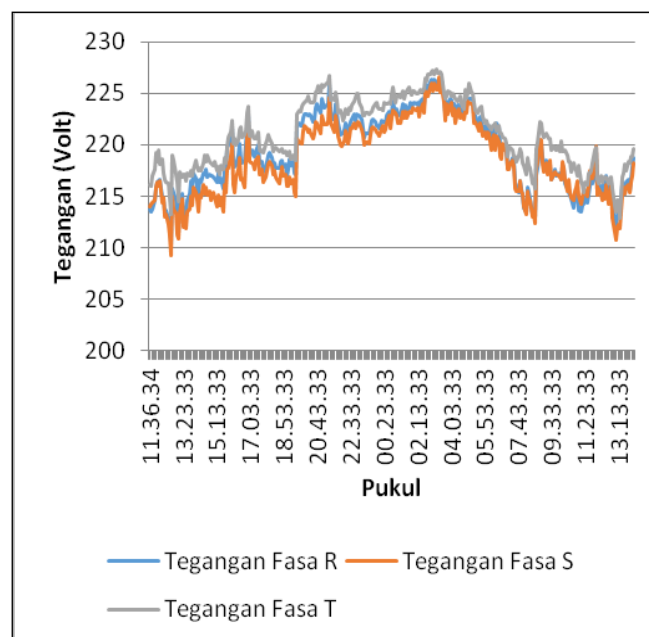
Figure 2. Graph of voltage measurement data per phase
