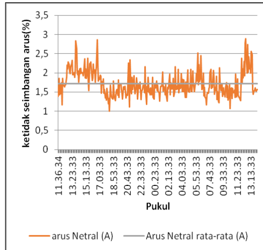
Figure 6. Graph of neutral currents due to current imbalance between phases
