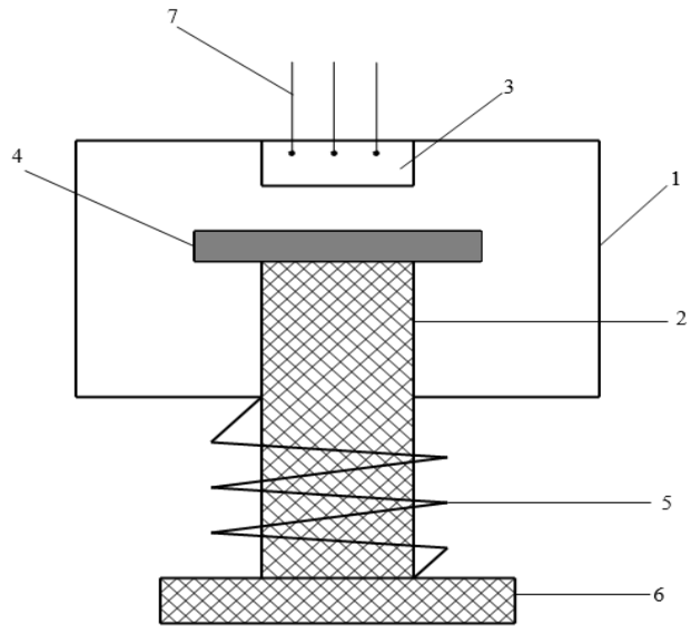
Figure 1. Scheme of the device using the Hall sensor. 1 – device case, 2 – pusher, 3 – Hall magnetik sensor, 4 – magnetized object, 5 – return spring, 6 – skin touching plate, 7-signal transmission cables.
