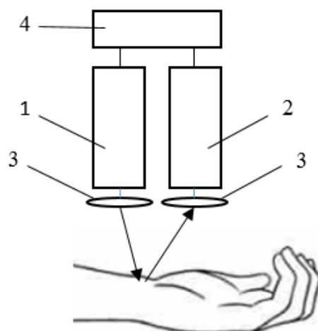
Figure 2. 1-Laser Beam Emitter, 2–laser beam receiver, 3-lens, 4-time interval measuring device.
