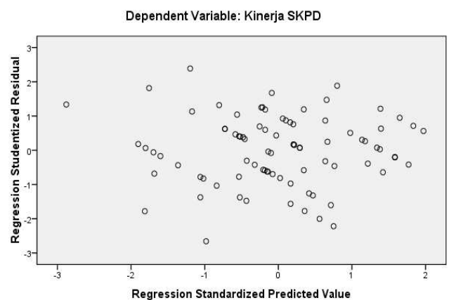
Scatterplot
